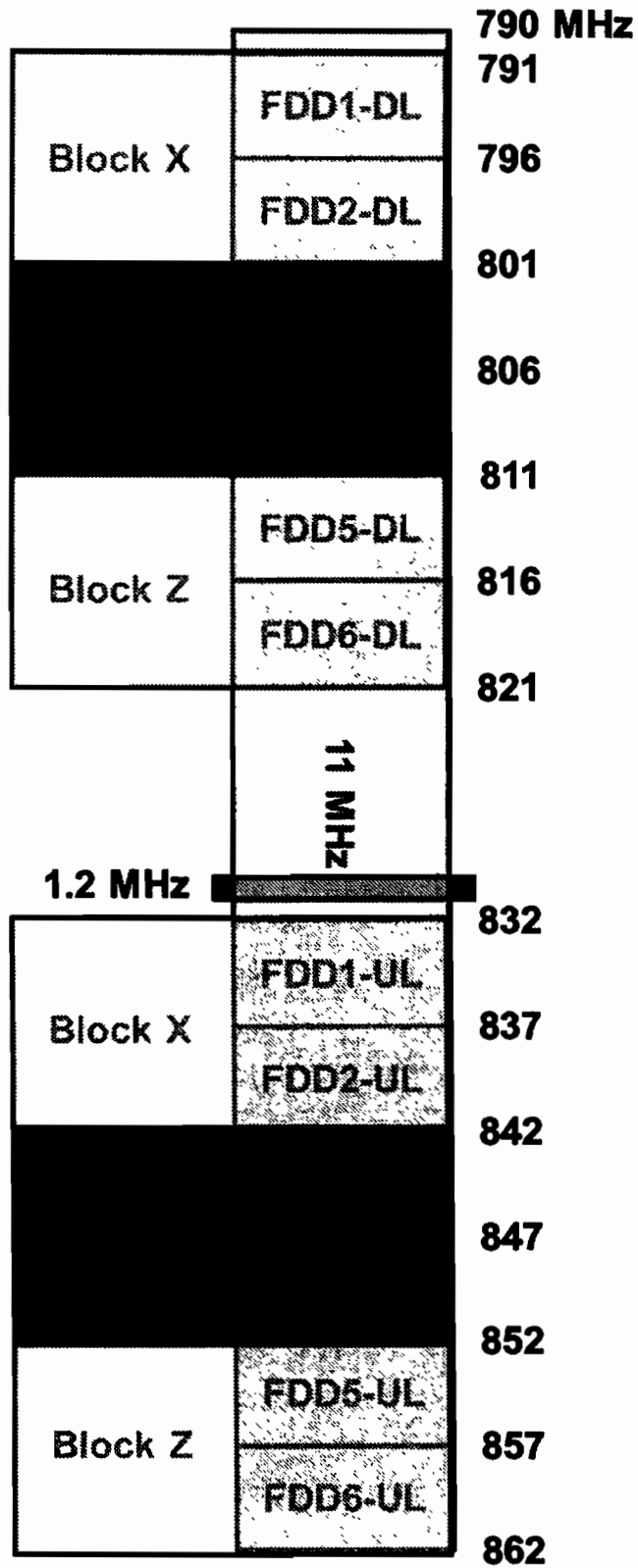
Figure 2: Spectrum licensing configuration for the 800 MHz band
